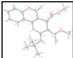
Fig. 1. The molecular structure of the title compound with the atom numbering scheme. Displacement ellipsoids are drawn at 30% probability level. H atoms are presented as small spheres of arbitrary radius.
