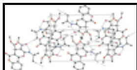
Fig. 2. The packing arrangement of the title compound viewed down c axis, showing formation of hydrogen bond. Dashed lines indicate the intramolecular N—H...O and intermolecular C—H...O interactions.
